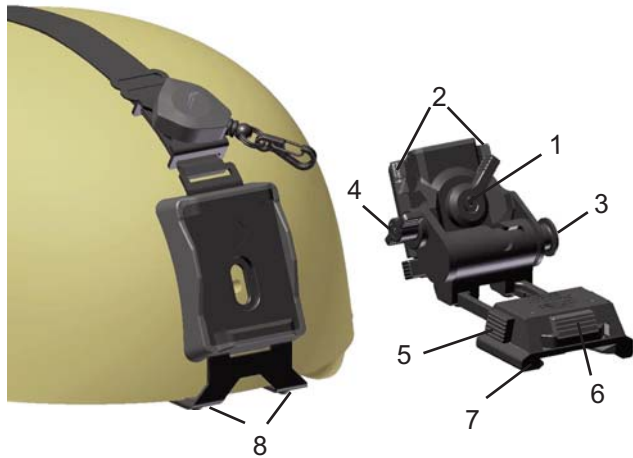
L4 G24 Mount with Low Profile Breakaway Base
